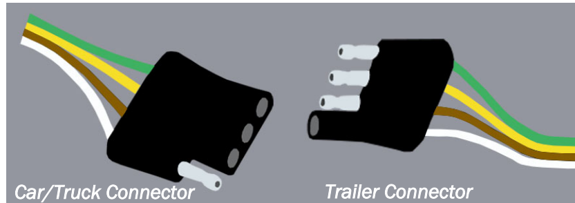
Figure 5.3.3A Four Pin Flat Connector
